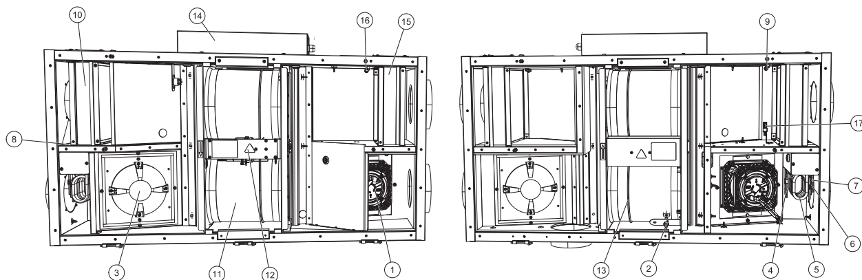
Fig. 10 Internal components
