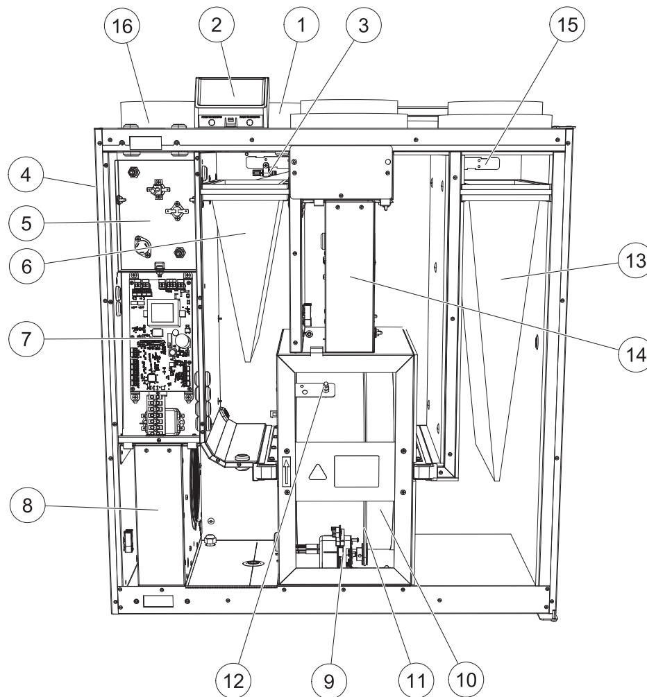
Fig. 10 Internal components
